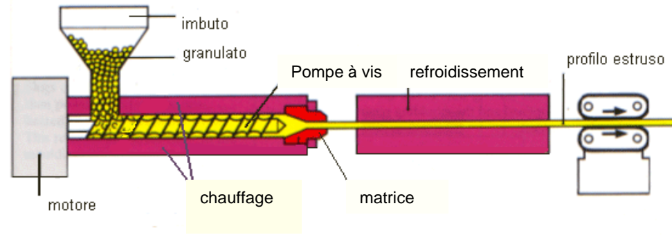
Extrusion
